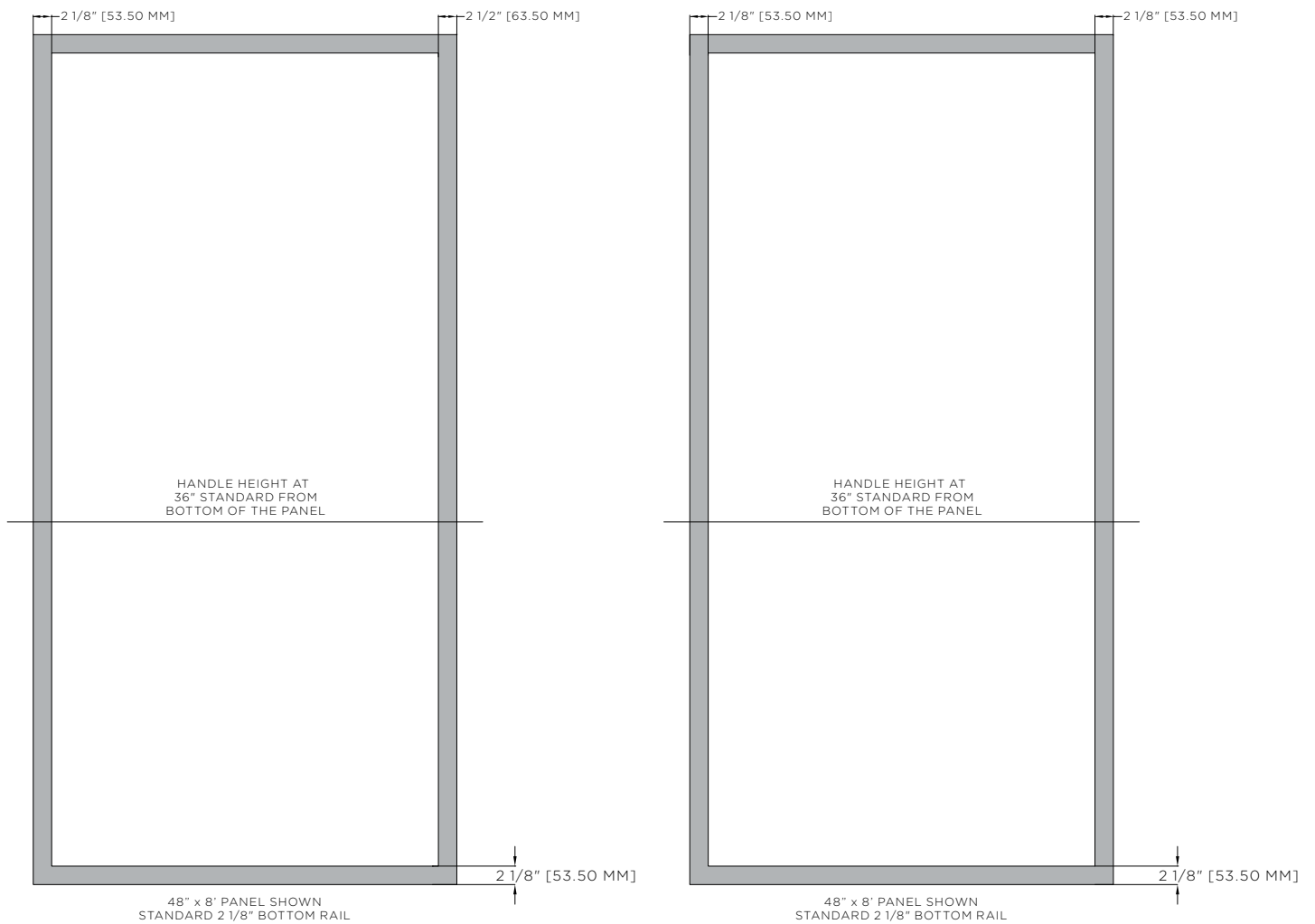
JAMB STILE CONDITION
