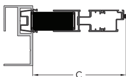
HORIZONTAL SECTION - JAMB STRIKE
