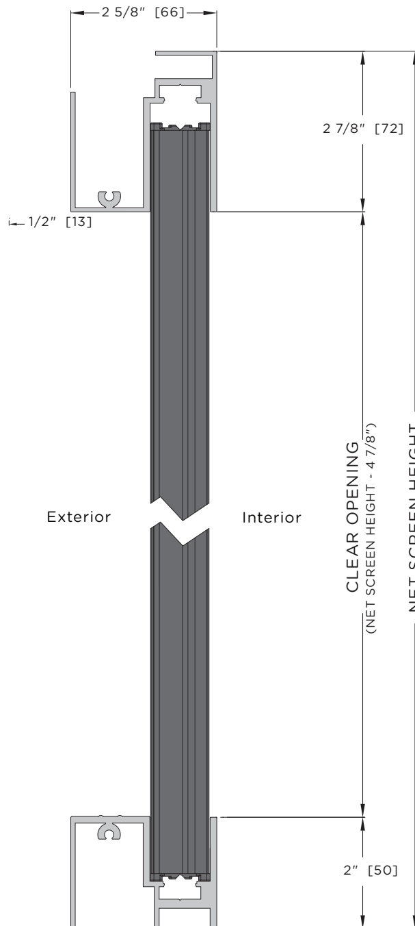
VERTICAL SECTION STANDARD
