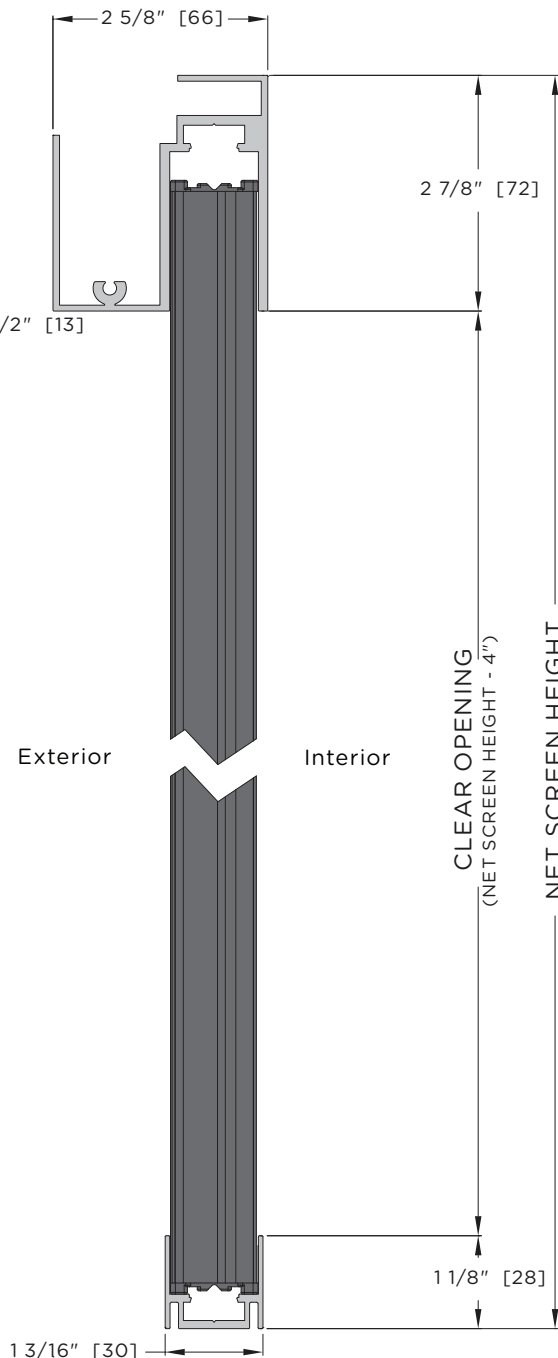
VERTICAL SECTION WITH LOW PROFILE SILL
