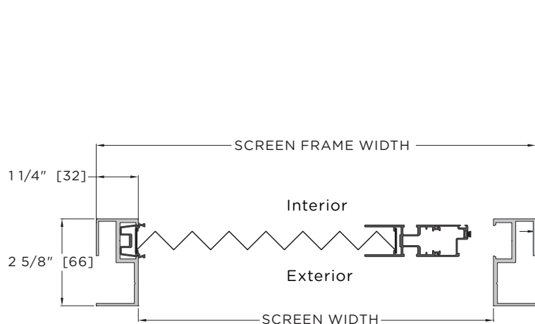
HORIZONTAL SECTION - JAMB STRIKE
