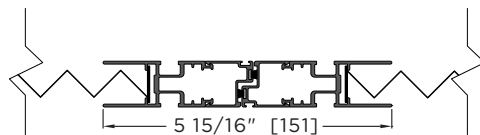
MEETING DETAIL DOUBLE SCREEN
